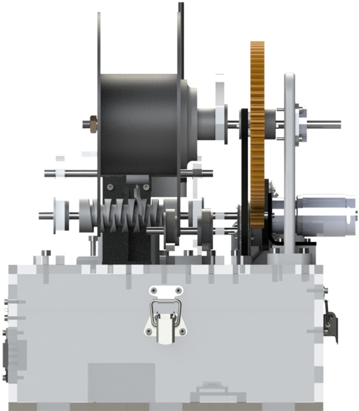
Gambar 5 - Tampak Samping Kiri
